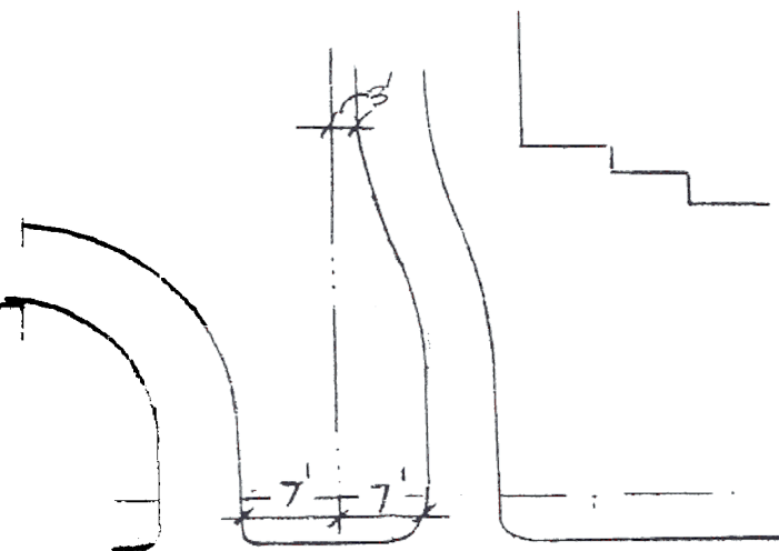
ADJACENT DRIVEWAYS
