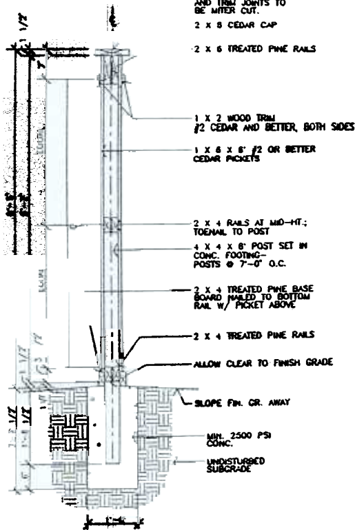
DOUBLE SIDED WOOD FENCE - SECTION
